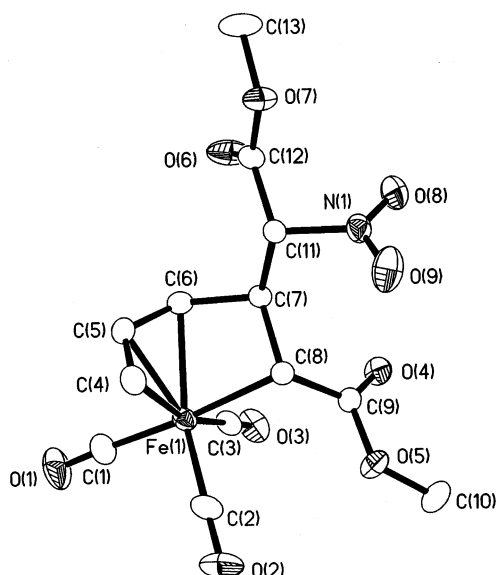
FIGURE 1. ORTEP representation of the X-ray crystal structure of 2d' . Selected bond lengths (Å): Fe(1)–C(4), 2.143(3); Fe(1)–C(5), 2.087(3); Fe(1)–C(6), 2.146(3); Fe(1)–C(8), 2.106(2); C(4)–C(5), 1.396(4); C(5)–C(6), 1.394(4); C(6)–C(7), 1.515(3); C(7)–C(8), 1.514(3).
